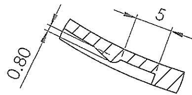
DETAIL C SCALE 2 : 1
